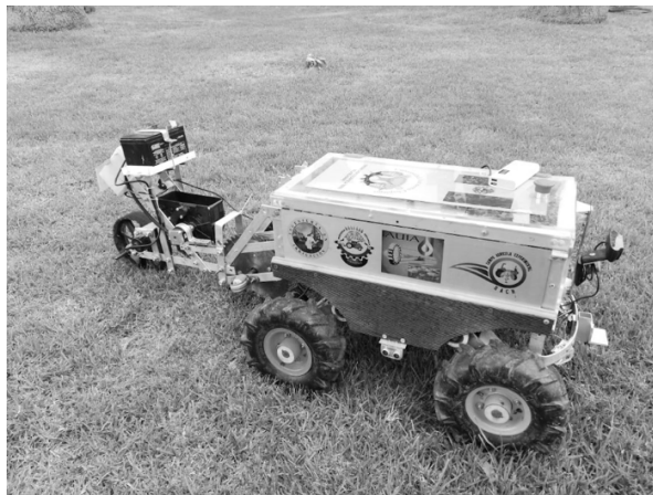
Figure 5. First agriculture robot named “Voltan”
