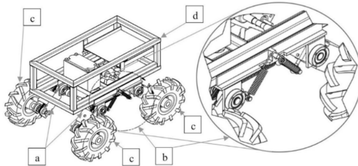
Figure 1. Suspension system. a) Support arms, c) Tires and d) Chassis
