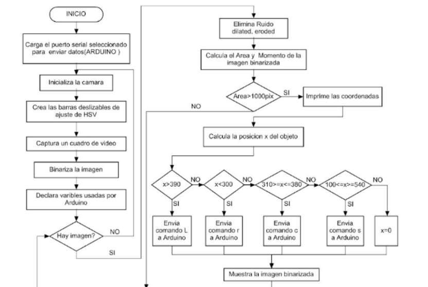
Figure 3. Flow diagram of the servo visual control implemented
