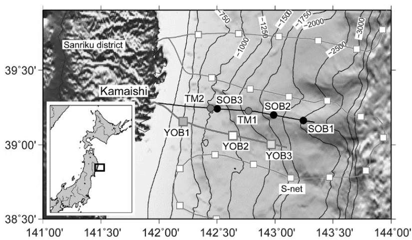
Figure 9. Positions of the deployed ITC system
