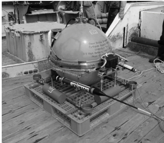
Figure 4. Photograph of the Broadband Ocean Bottom Seismometer (BBOBS) before deployment
