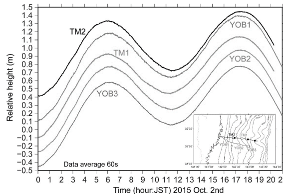
Figure 11. Records from pressure gauge by the OBCST system and the existing system
