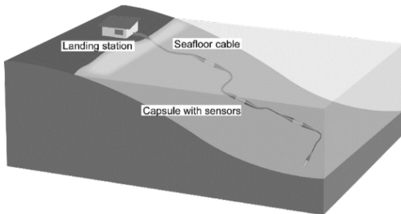
Figure 5. Schema of seafloor cabled observation system
