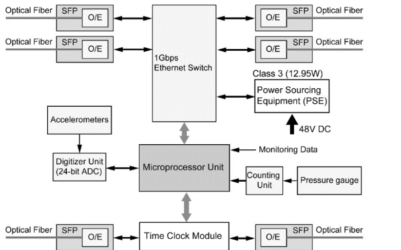
Figure 7. System block diagram of the observation unit for the OBCST system
