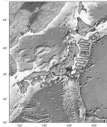
Figure 6. Positions of seafloor cabled stations around Japan as of March 2019
