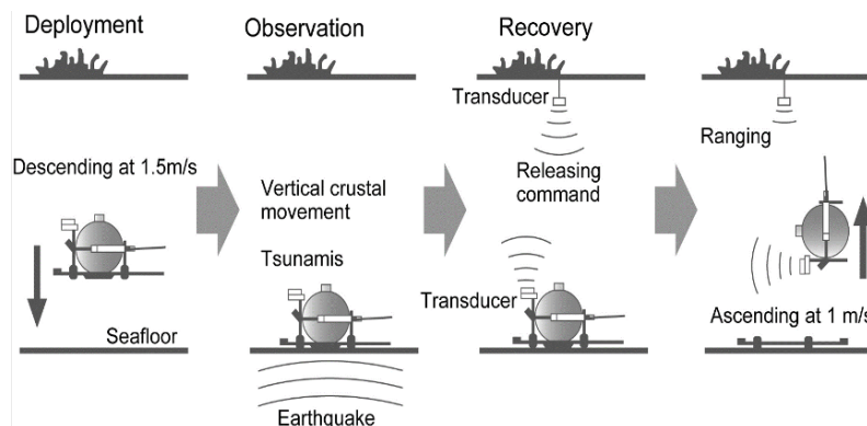
Figure 1. Schema of seafloor observation using free-fall pop-up type ocean bottom seismometer and/or pressure gauge
