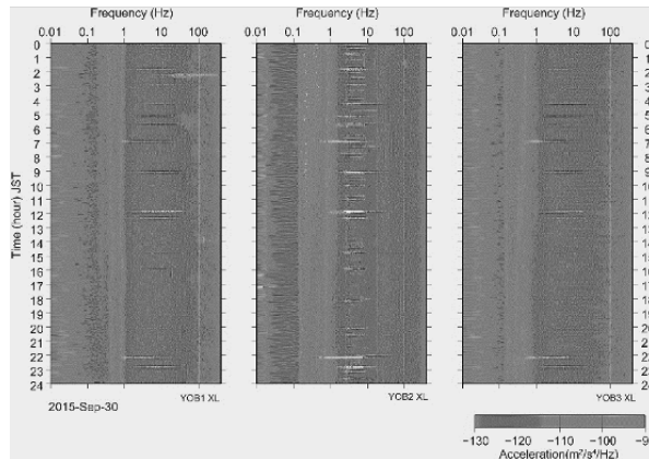
Figure 10. Running spectra of the records from the OBCST system. Spectra were calculated using one-day records on September 30th, 2015
